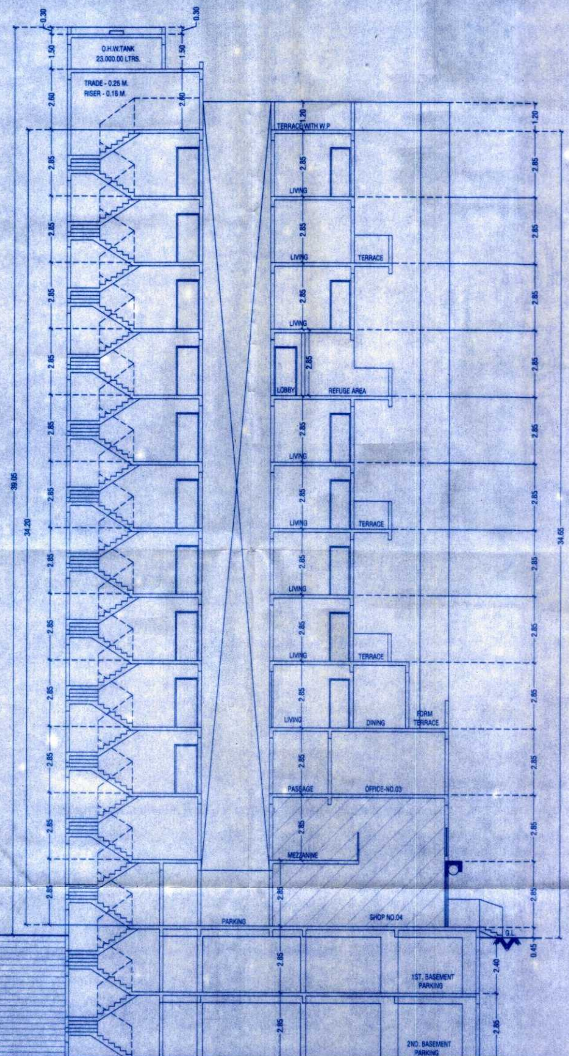
SECTION AT A-A'
