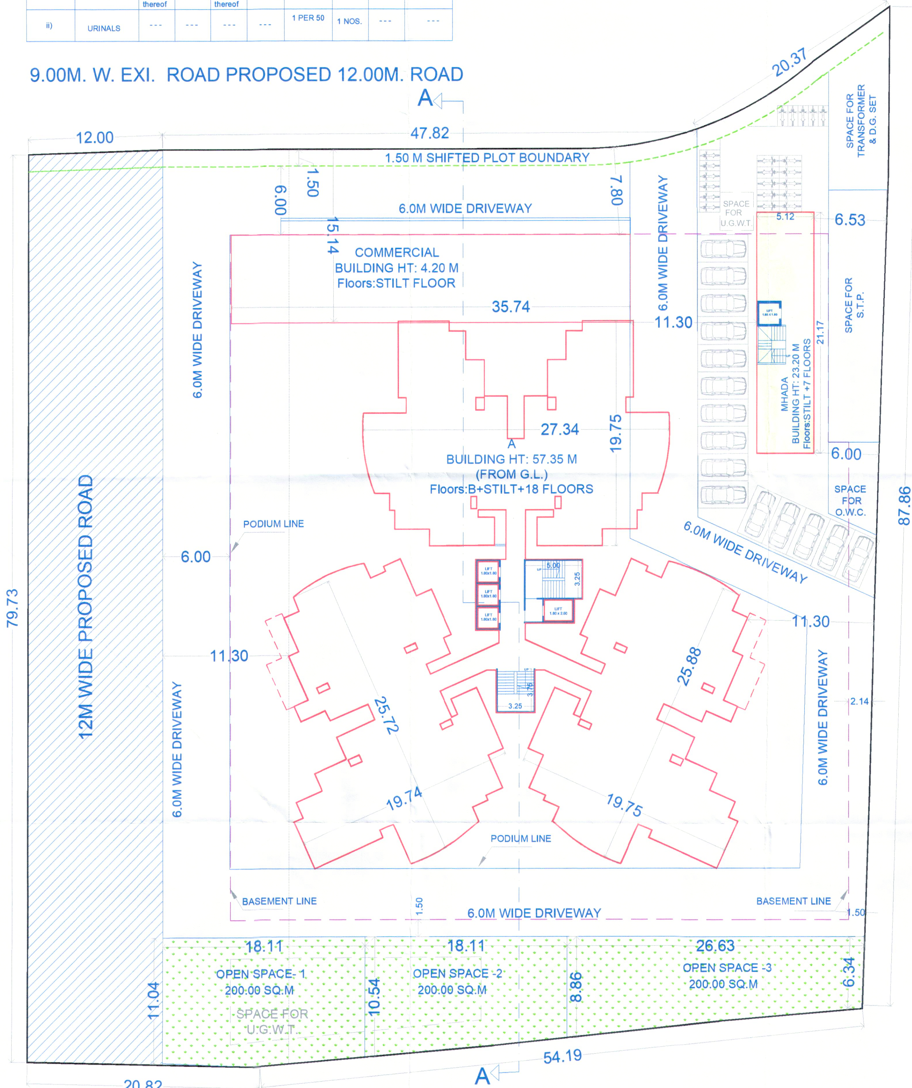
LOCATION PLAN (SCALE:1:200)
