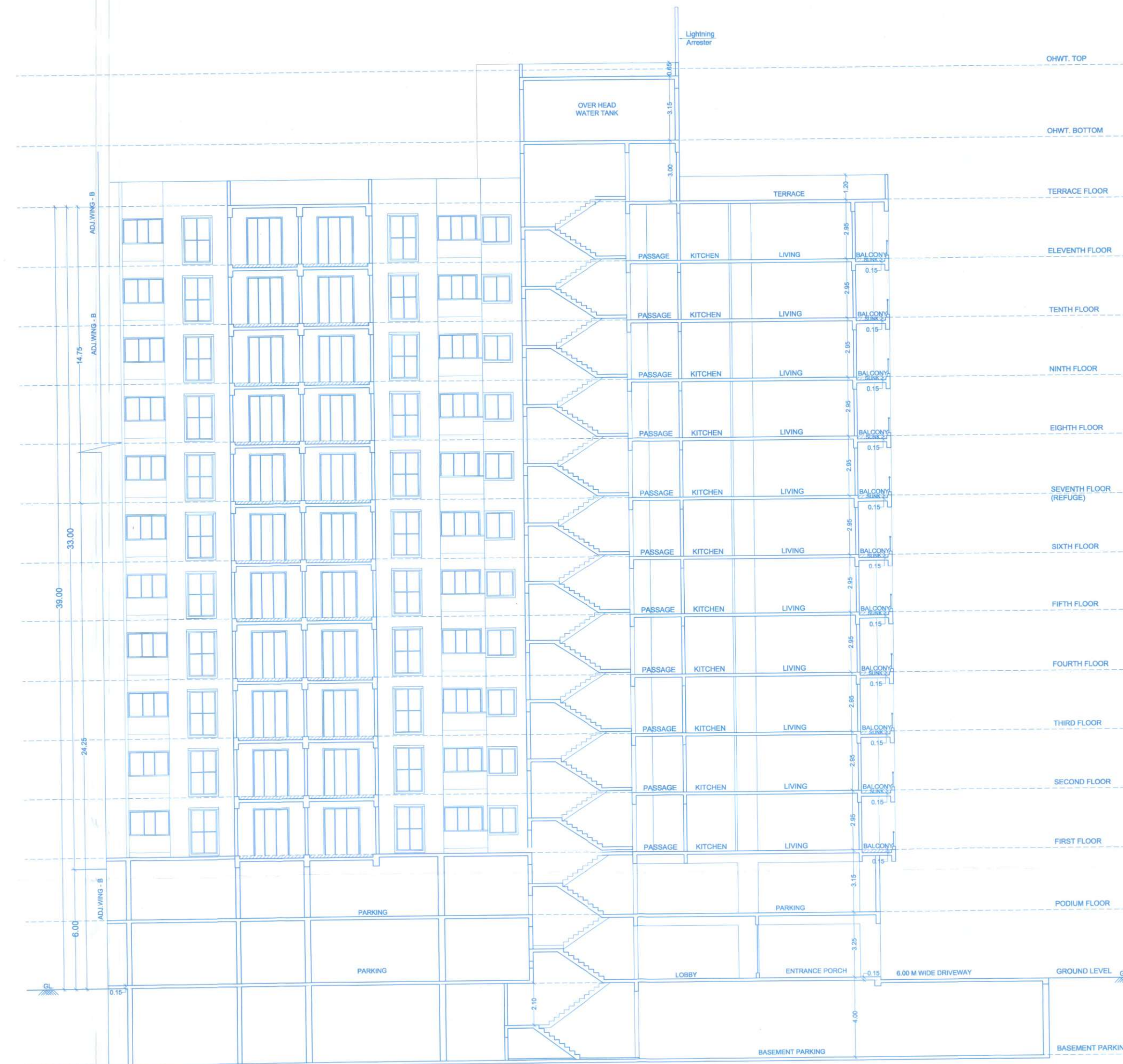
SECTION E-E SCALE 1:100
