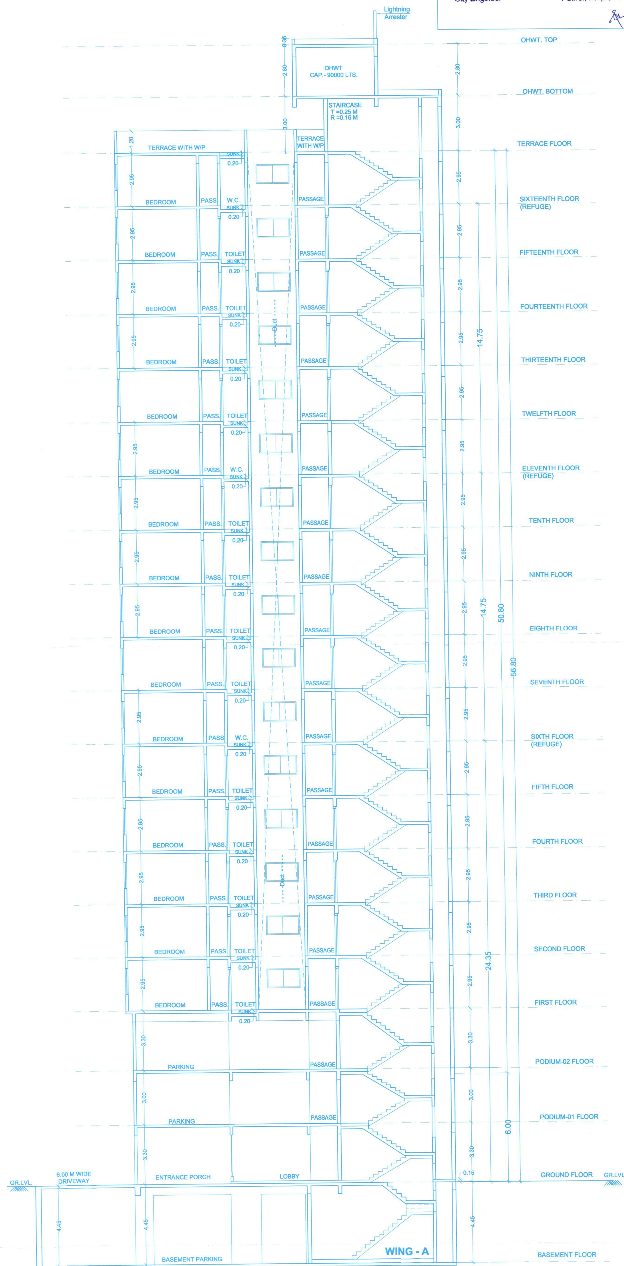
SECTION B - B SCALE 1:100
