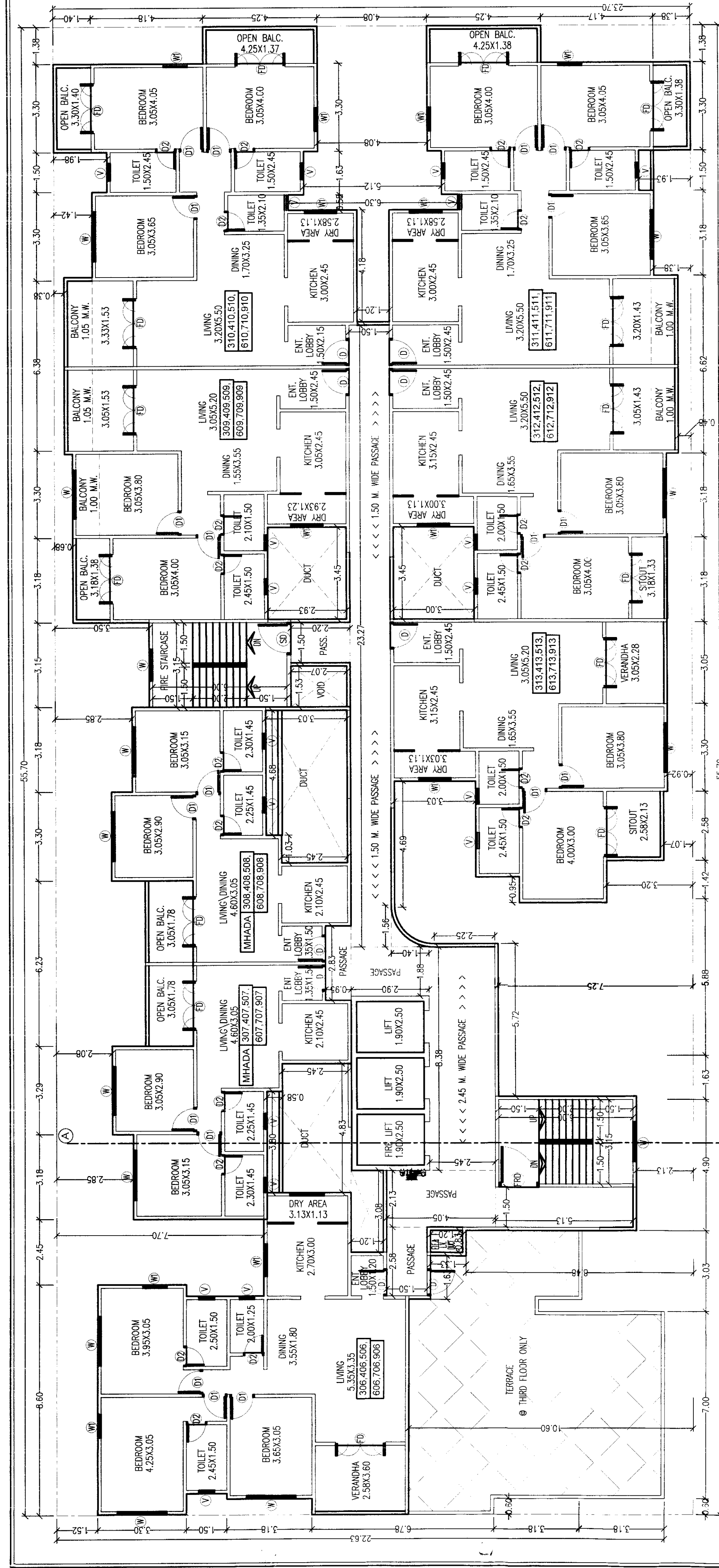
THIRD, FOURTH, FIFTH, SIXTH, SEVENTH, NINTH FLOOR PLAN
