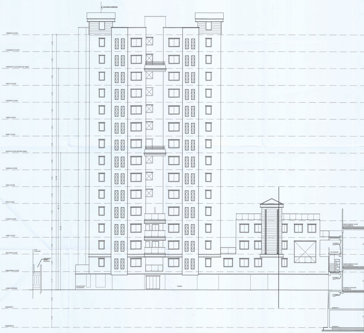
ROAD SIDE ELEVATION
