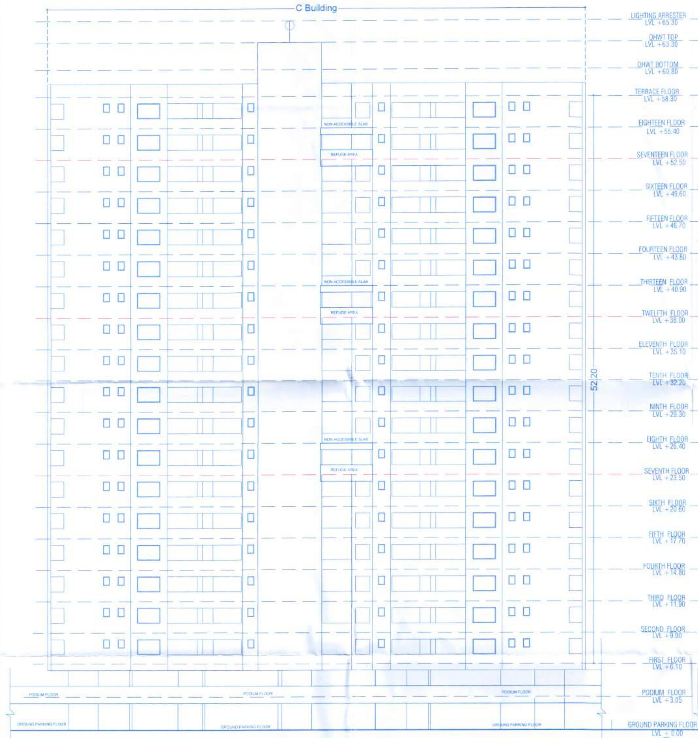
C BUILDING_ELEVATION (NTS)
