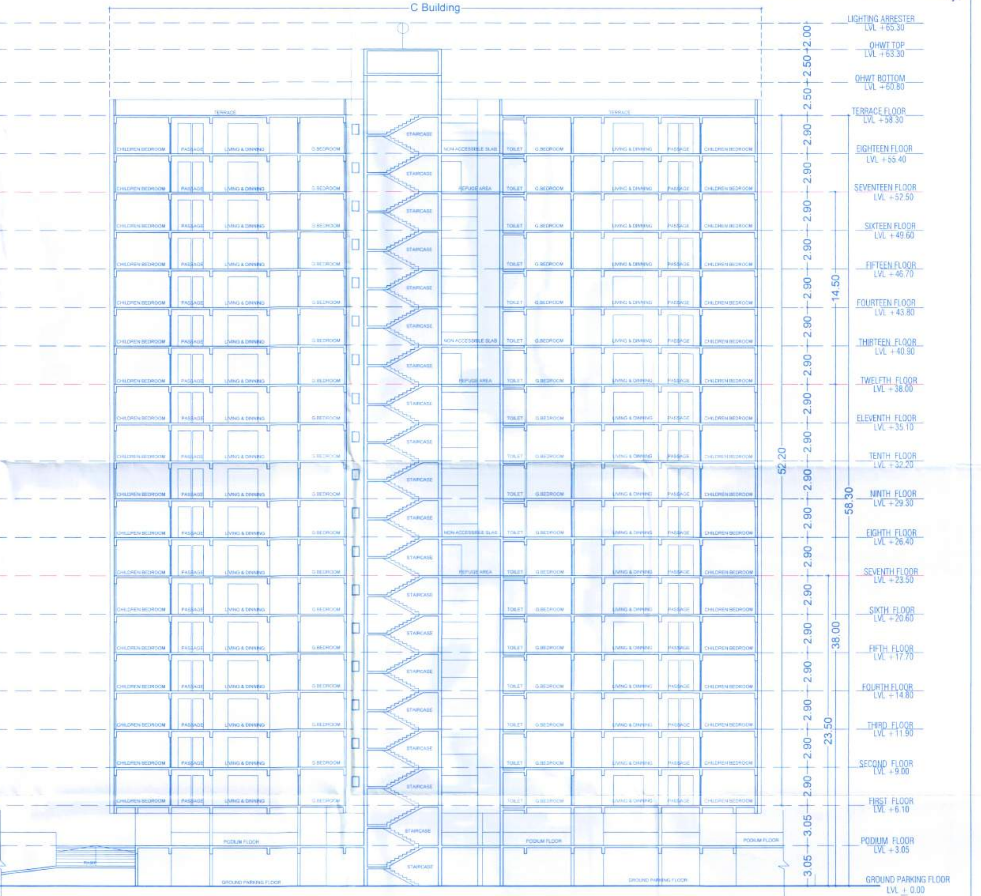
C BUILDING_SECTION CC (NTS)
