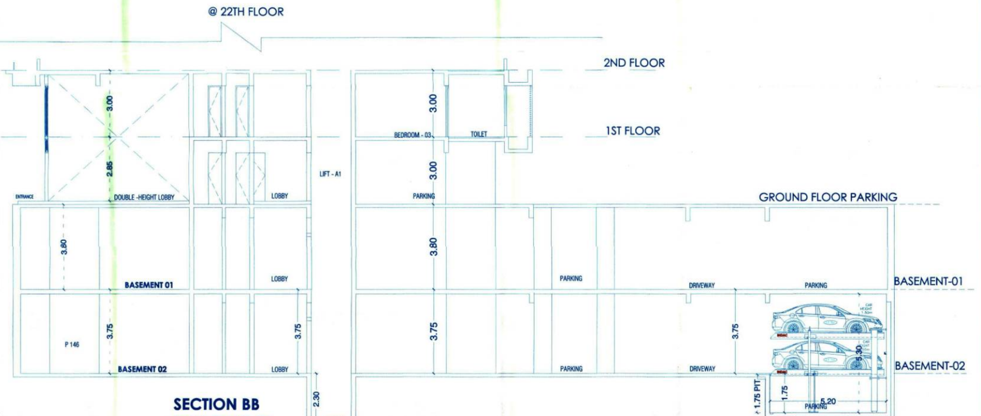
SECTION BB (BUILDING-B)
