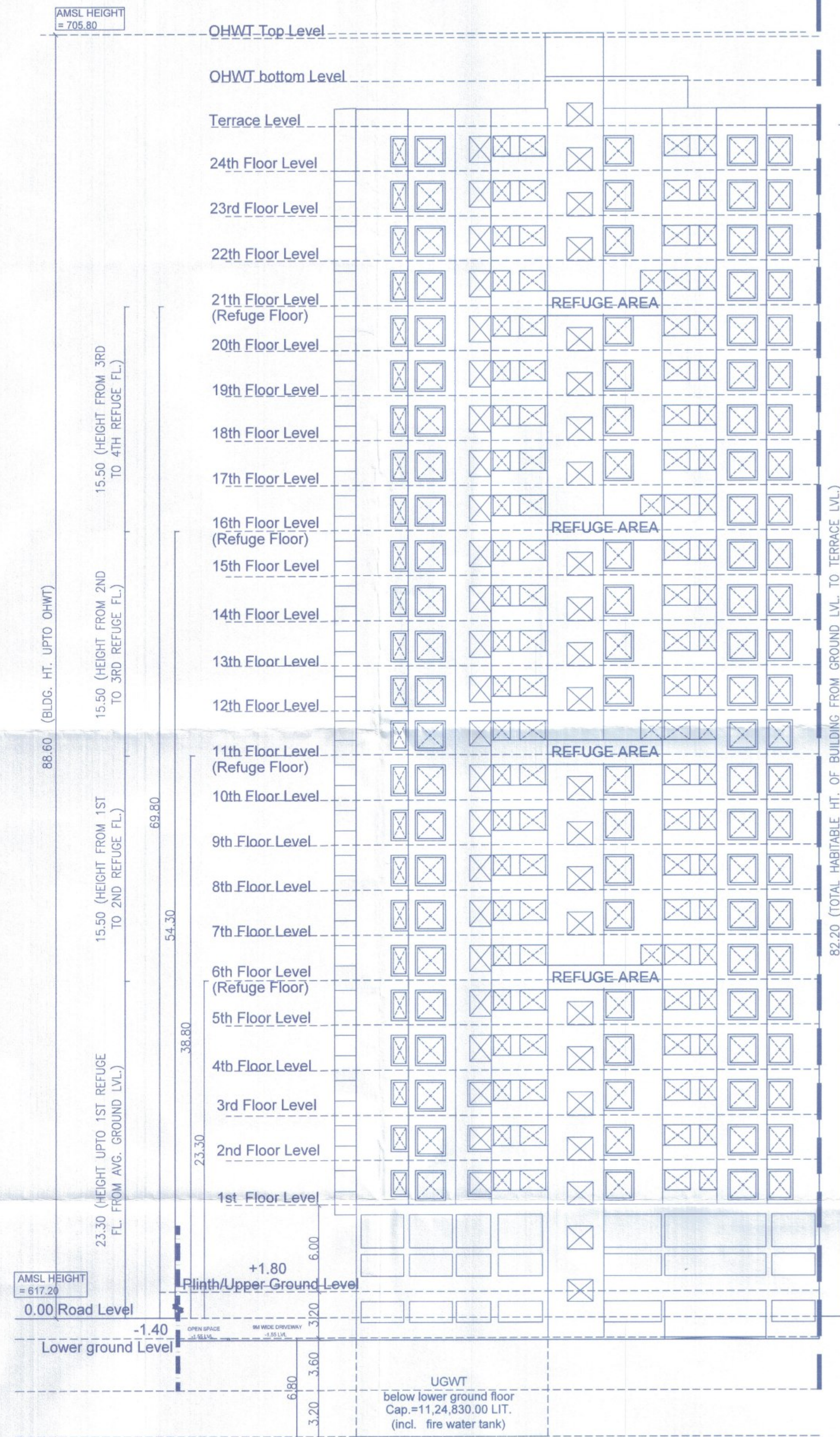
ELEVATION H WING D LG+UG+ 24 Floors 82.20 MT.
