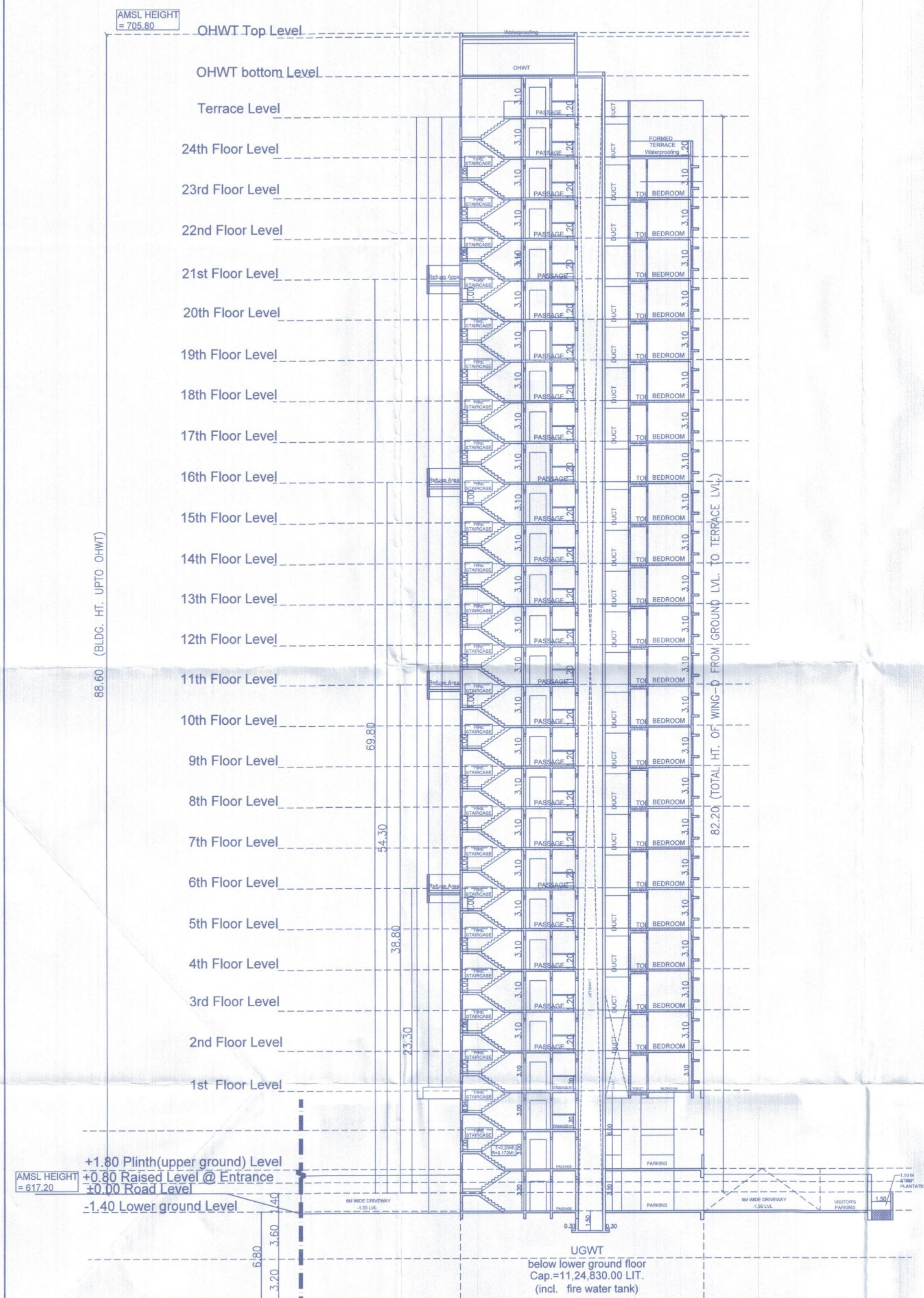
SECTION GG WING D LG+UG+ 24 Floors 82.20 MT.
