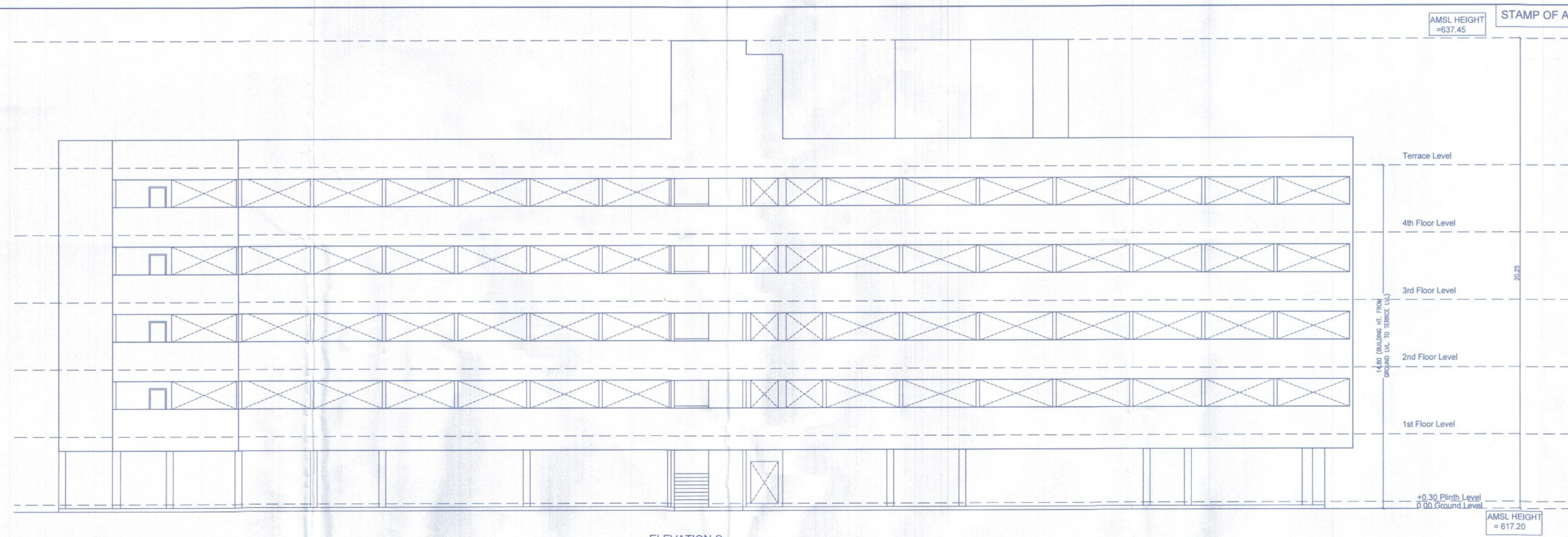
ELEVATION C RESERVATION BUILDING A WING + B WING P + 4 (HT.=14.80MT.)
