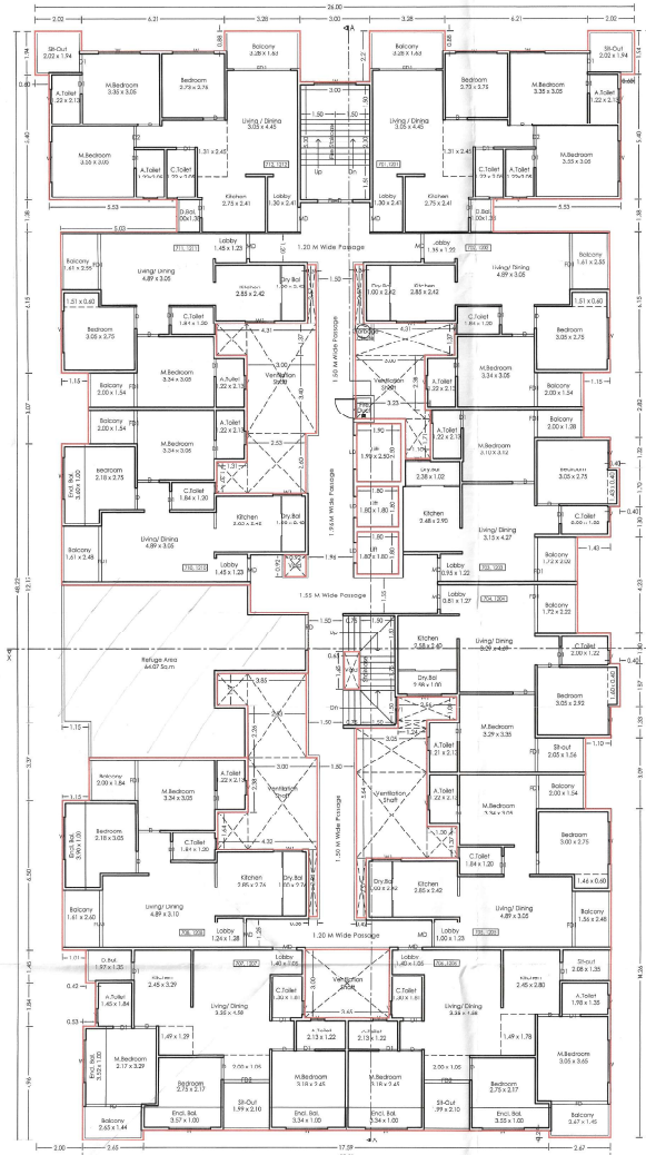
7TH & 12TH (REFUGE) FLOOR PLAN (WING - A)
