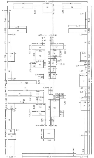
P-LINE DIAGRAM TYPICAL 7TH & 12TH (REFUGE) FLOOR PLAN (WING-A)
