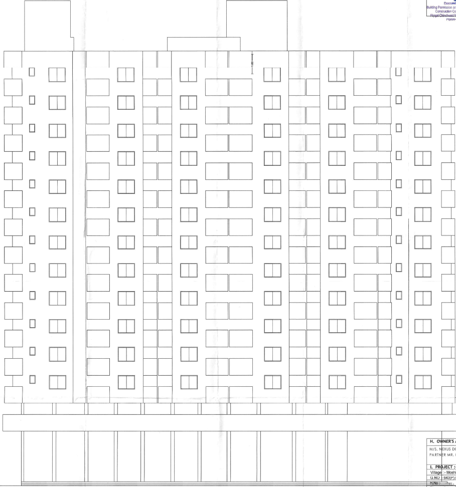
WEST SIDE ELEVATION (A - WING)
