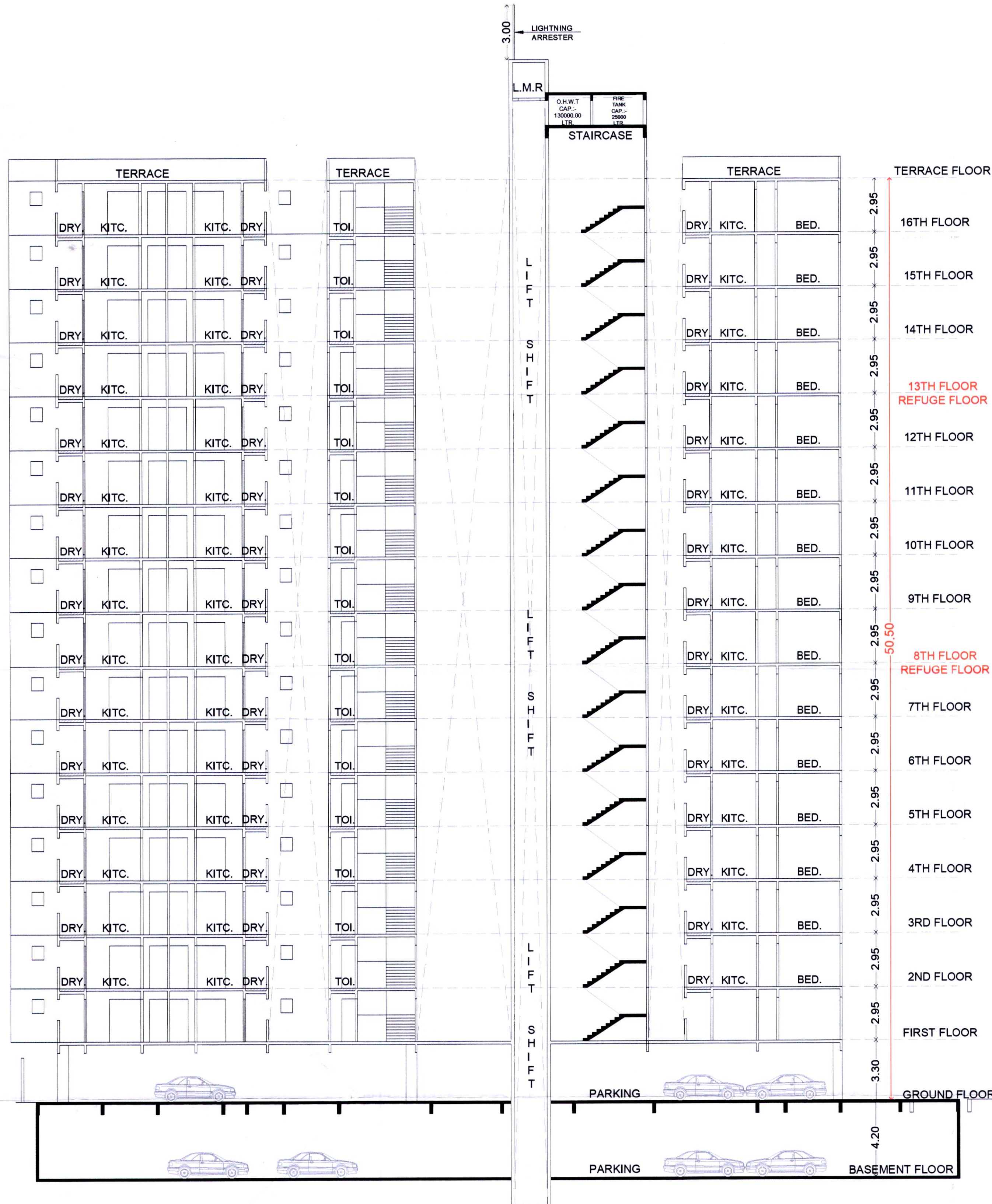
SECTION AA (WING B) (SCALE:-1:200)
