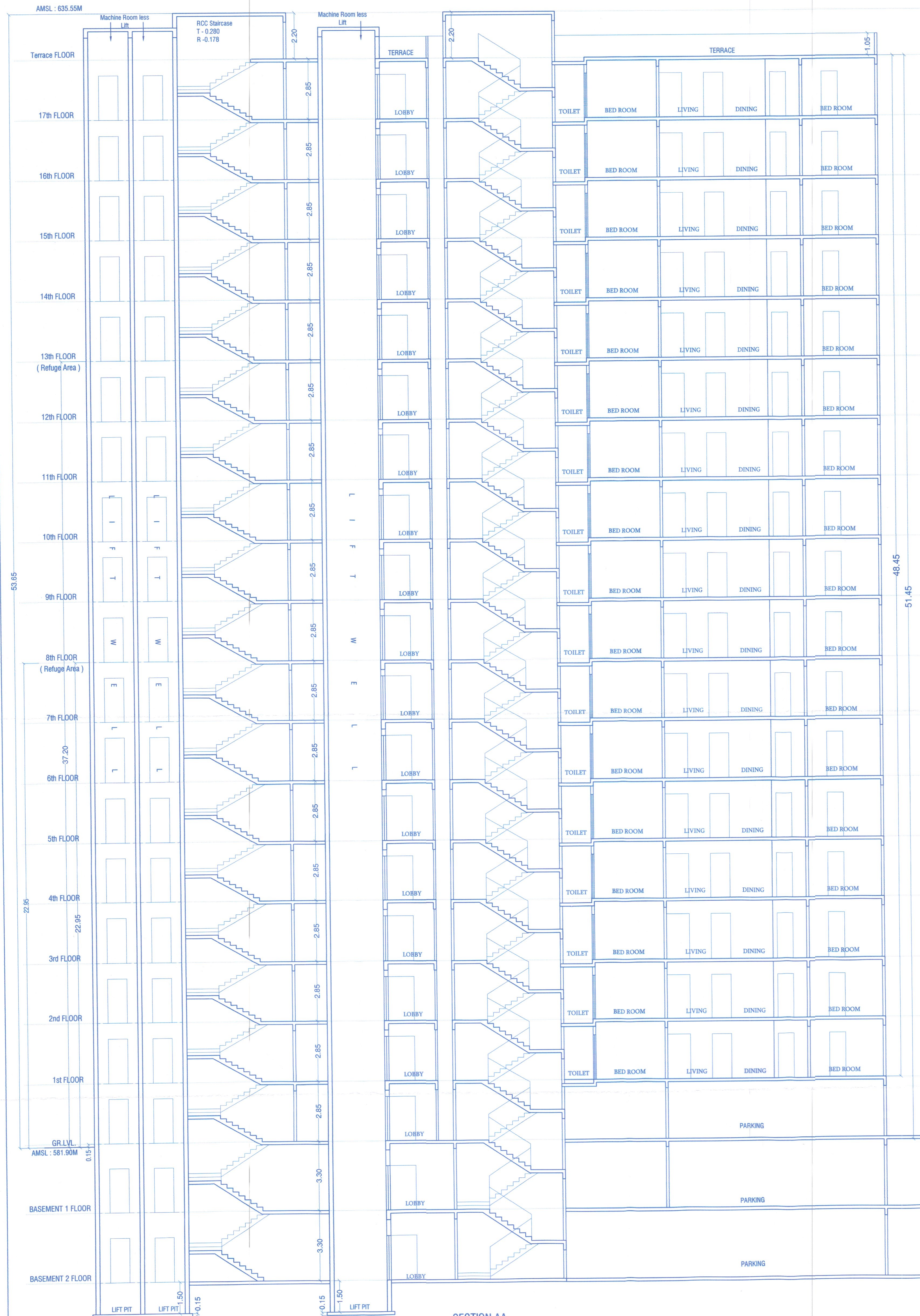
SECTION AA
