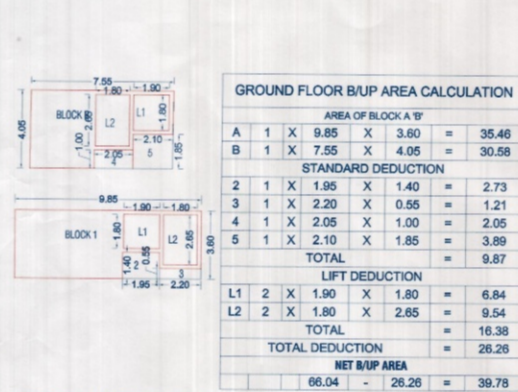
GROUND FLOOR AREA KEY PLAN SCALE 1:200 (A BUILDING)
