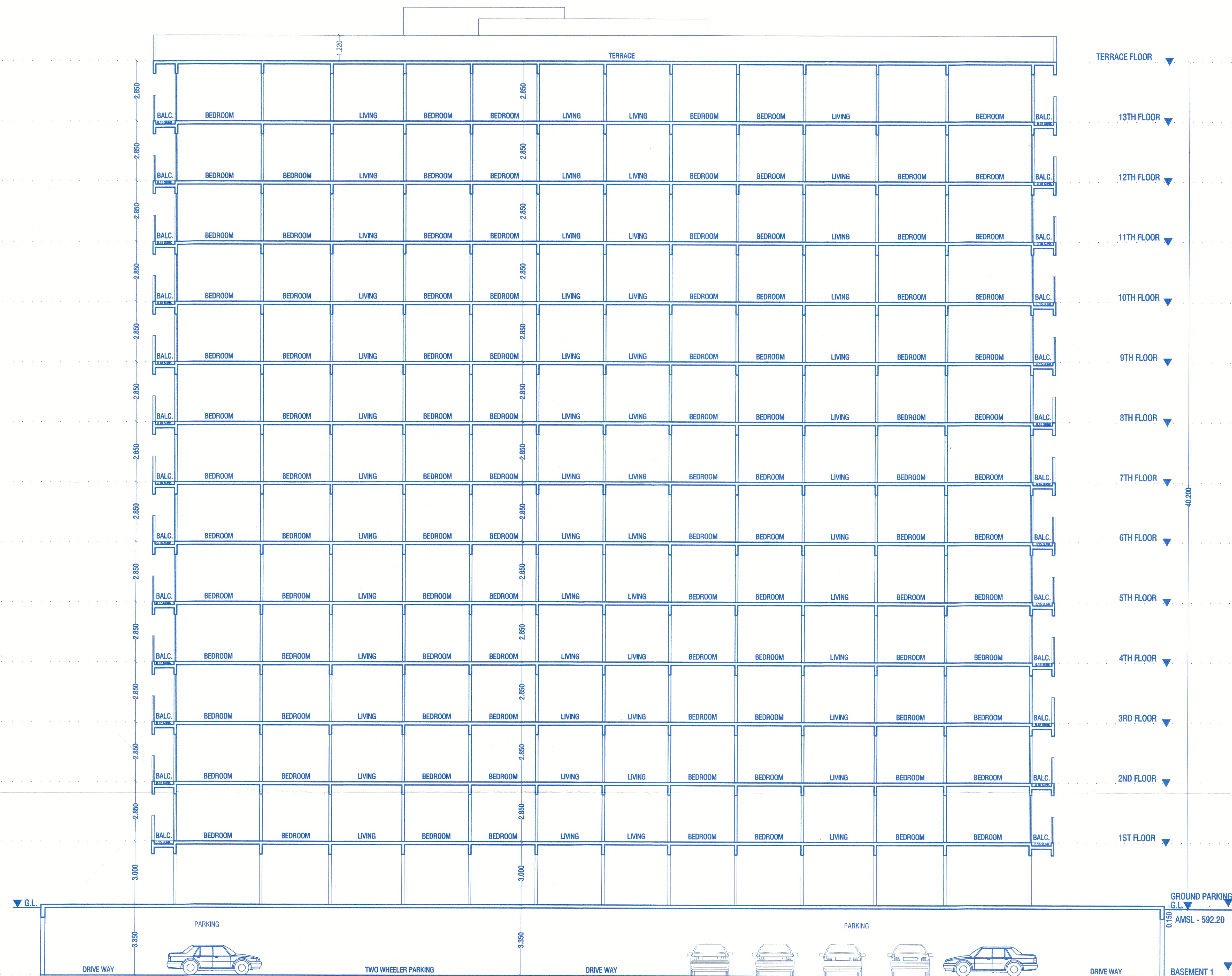
SECTION BB
