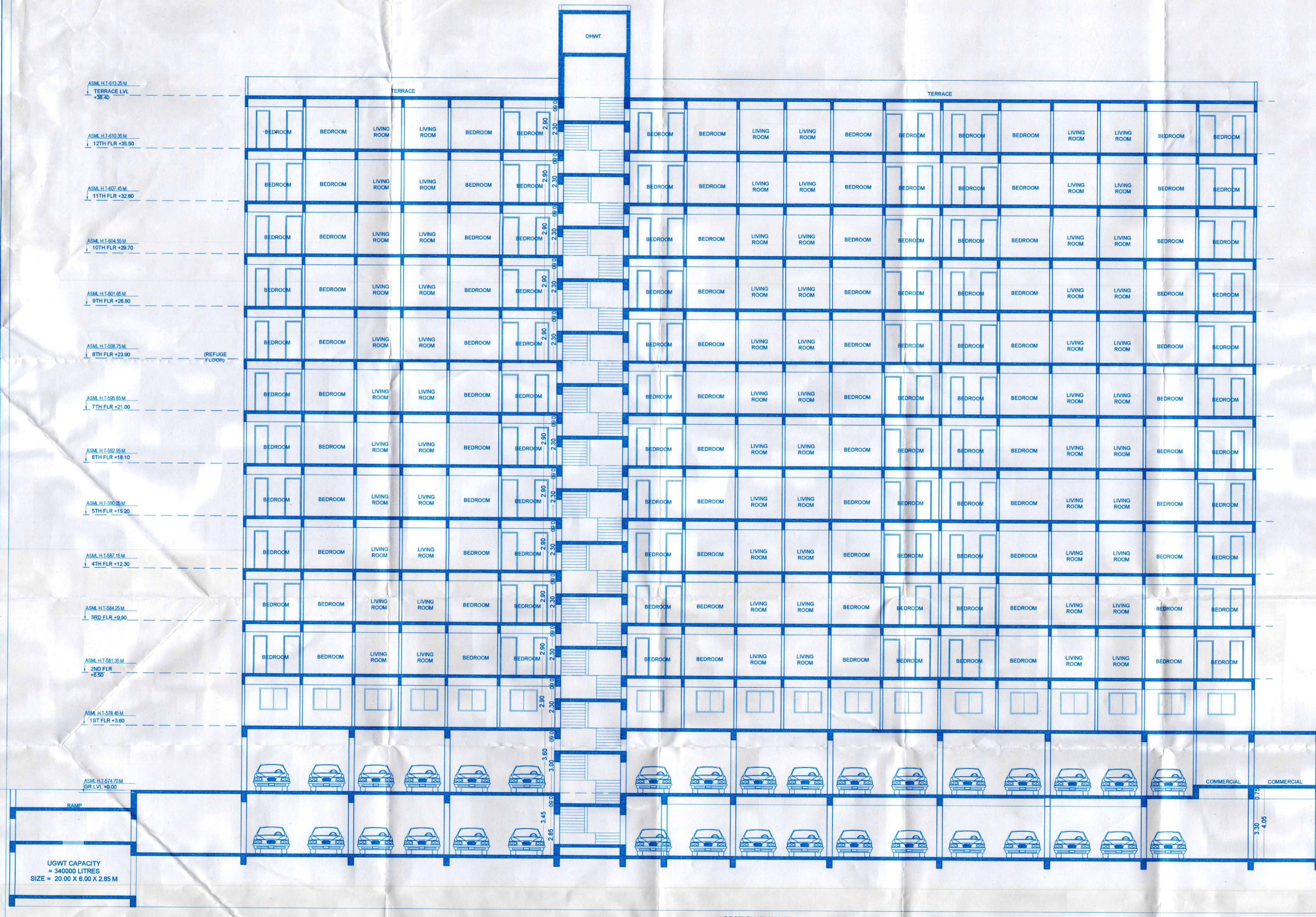
SECTION 'D' WING
