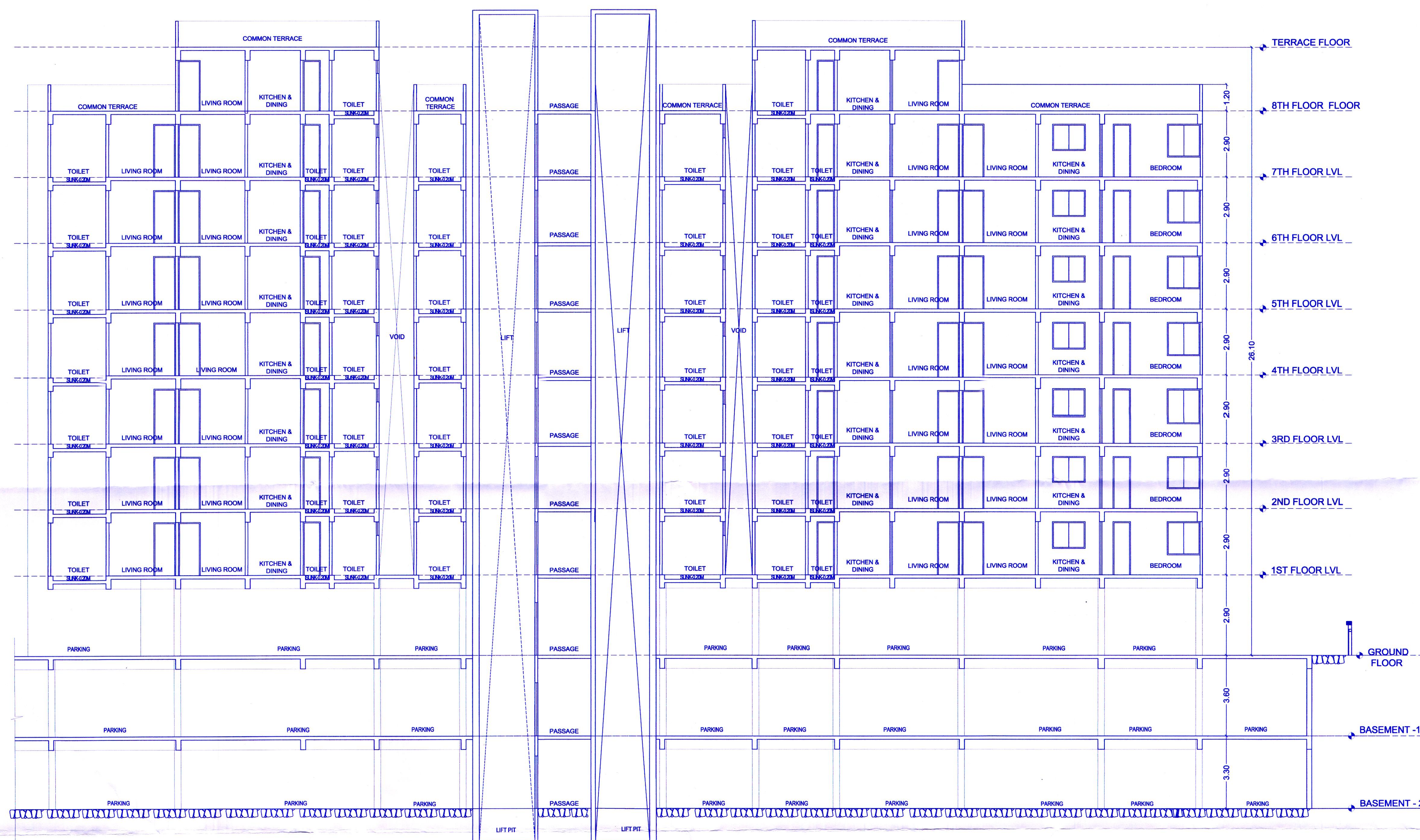
SECTION AT AA' SCALE - 1:100
