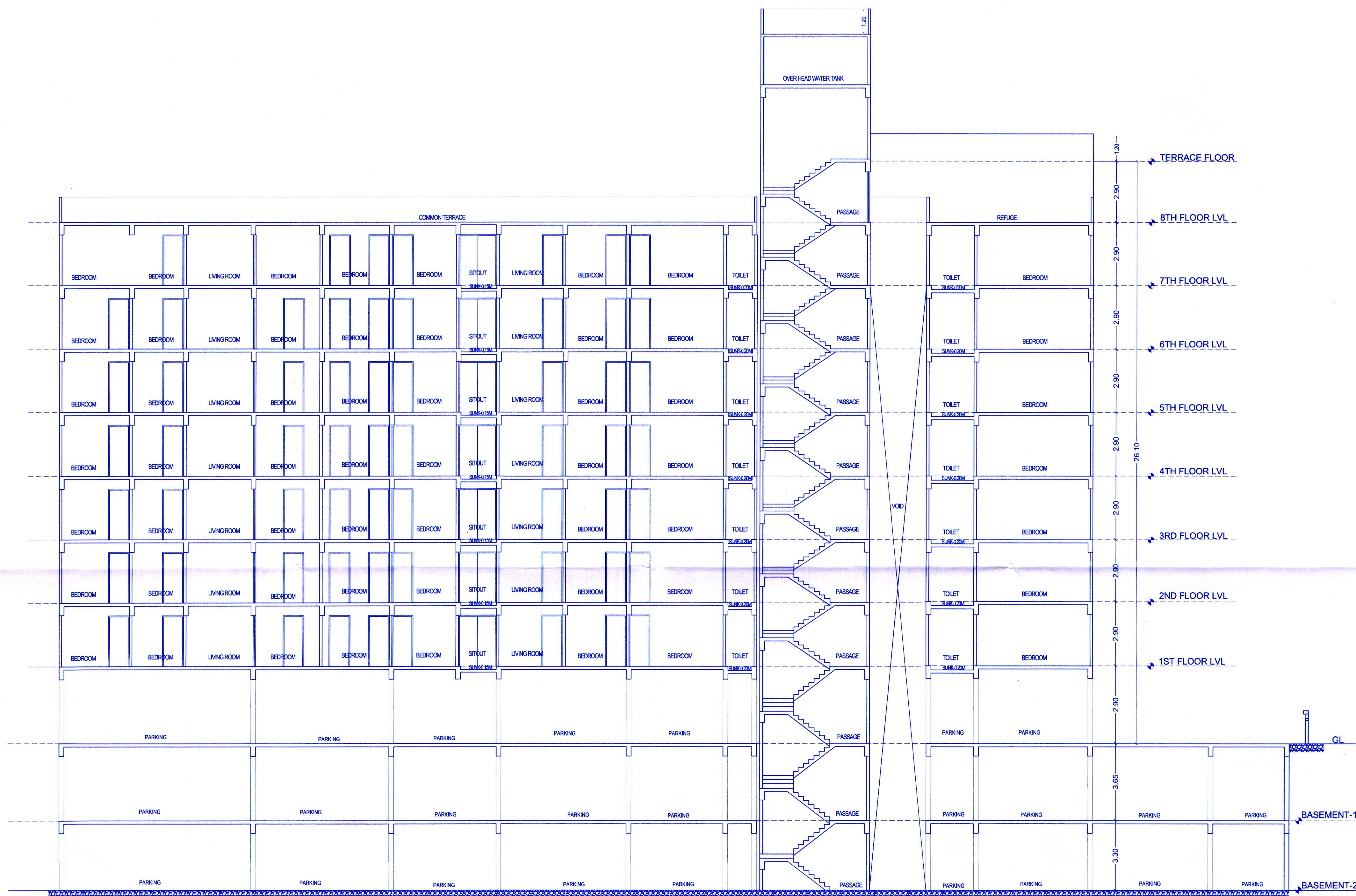
SECTION AT BB' SCALE - 1:100
