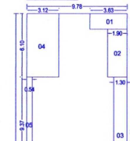
AREA DIAGRAM FOR SECOND FLOOR PLAN(MHADA) SCALE - 1:200
