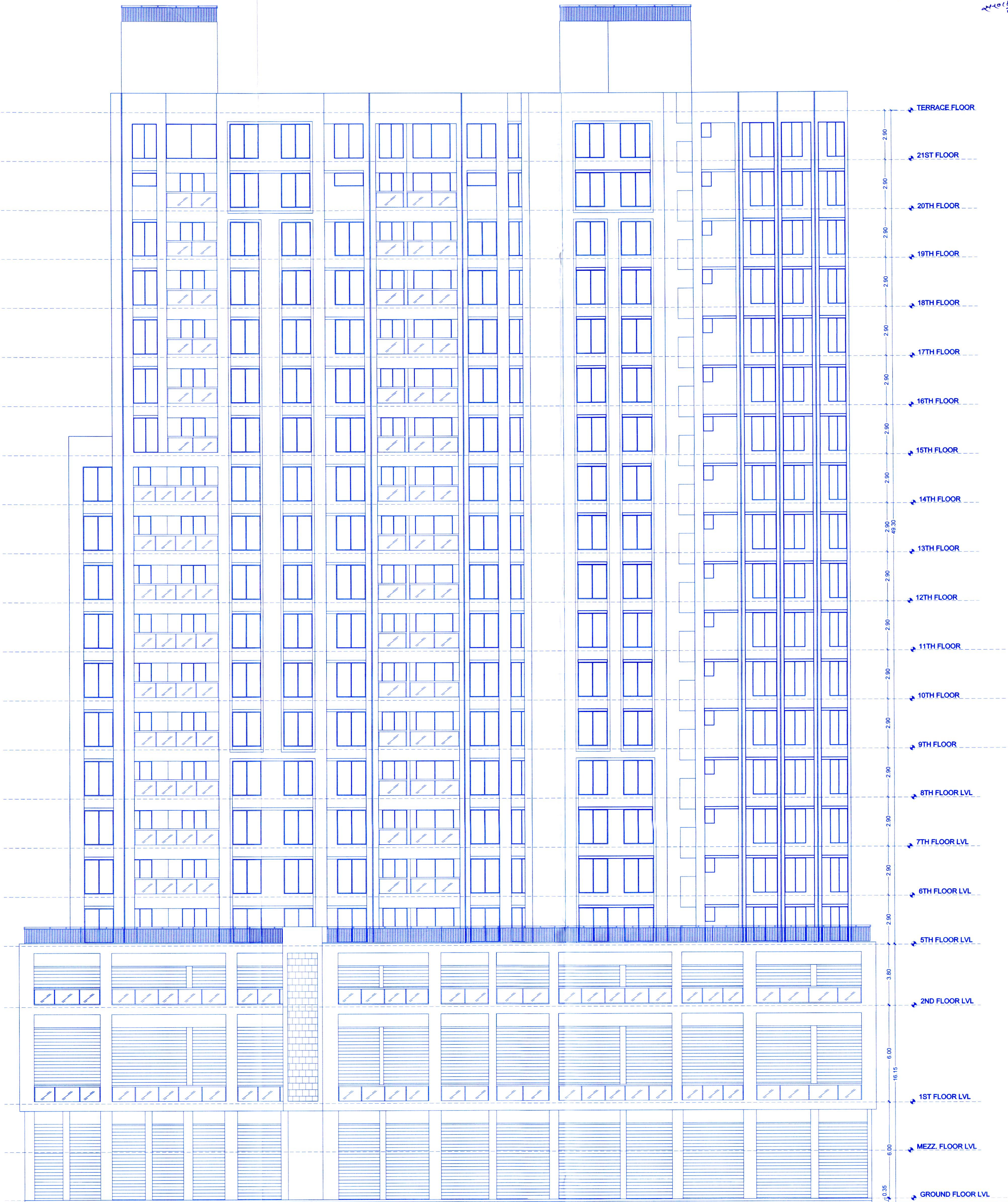
ELEVATION SCALE - 1:100
