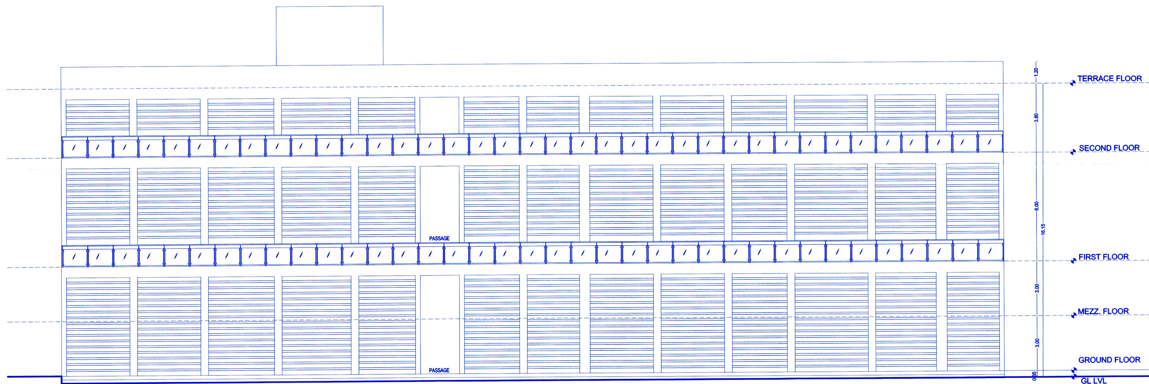
ELEVATION SCALE - 1:100
