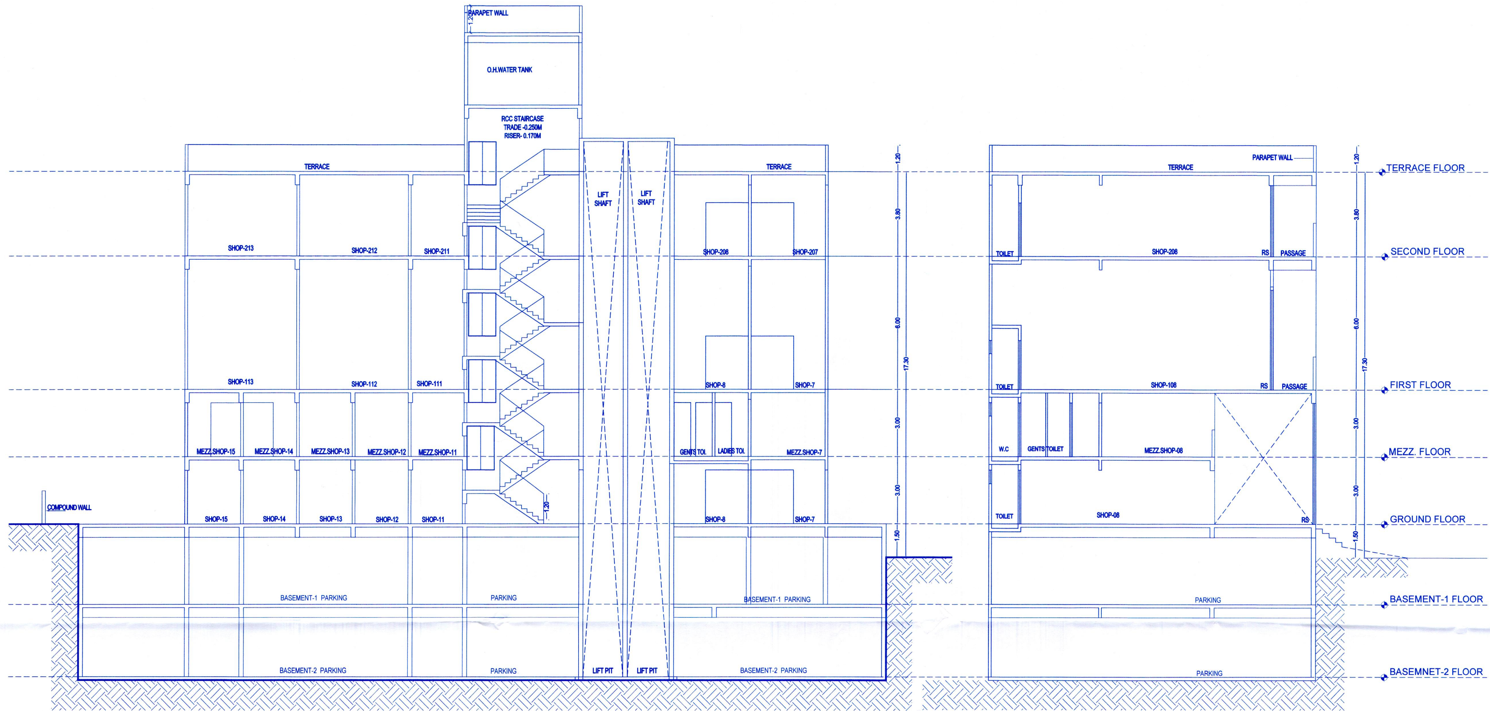
SECTION AT- AA SCALE - 1:100
