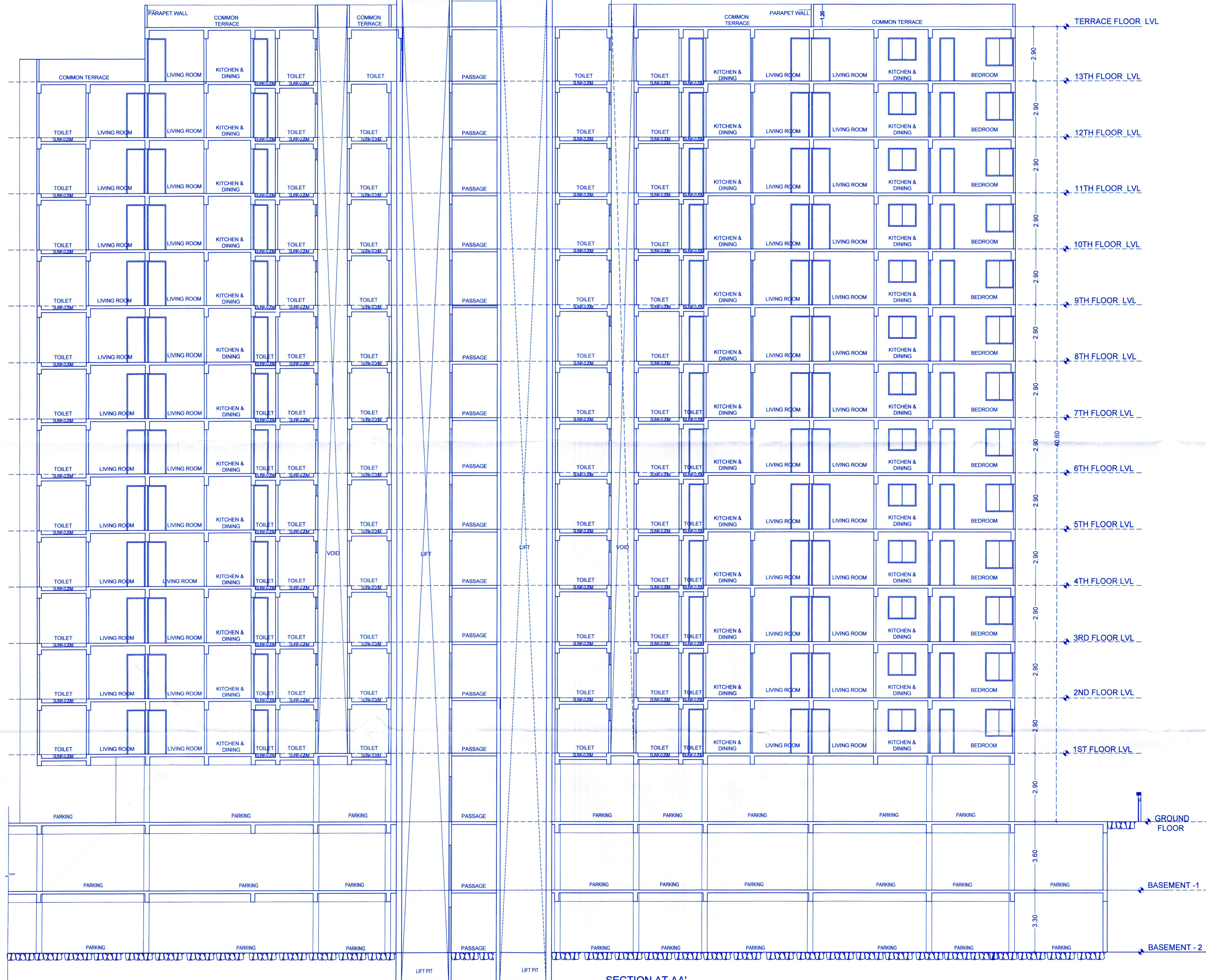
SECTION AT AA' SCALE - 1:100
