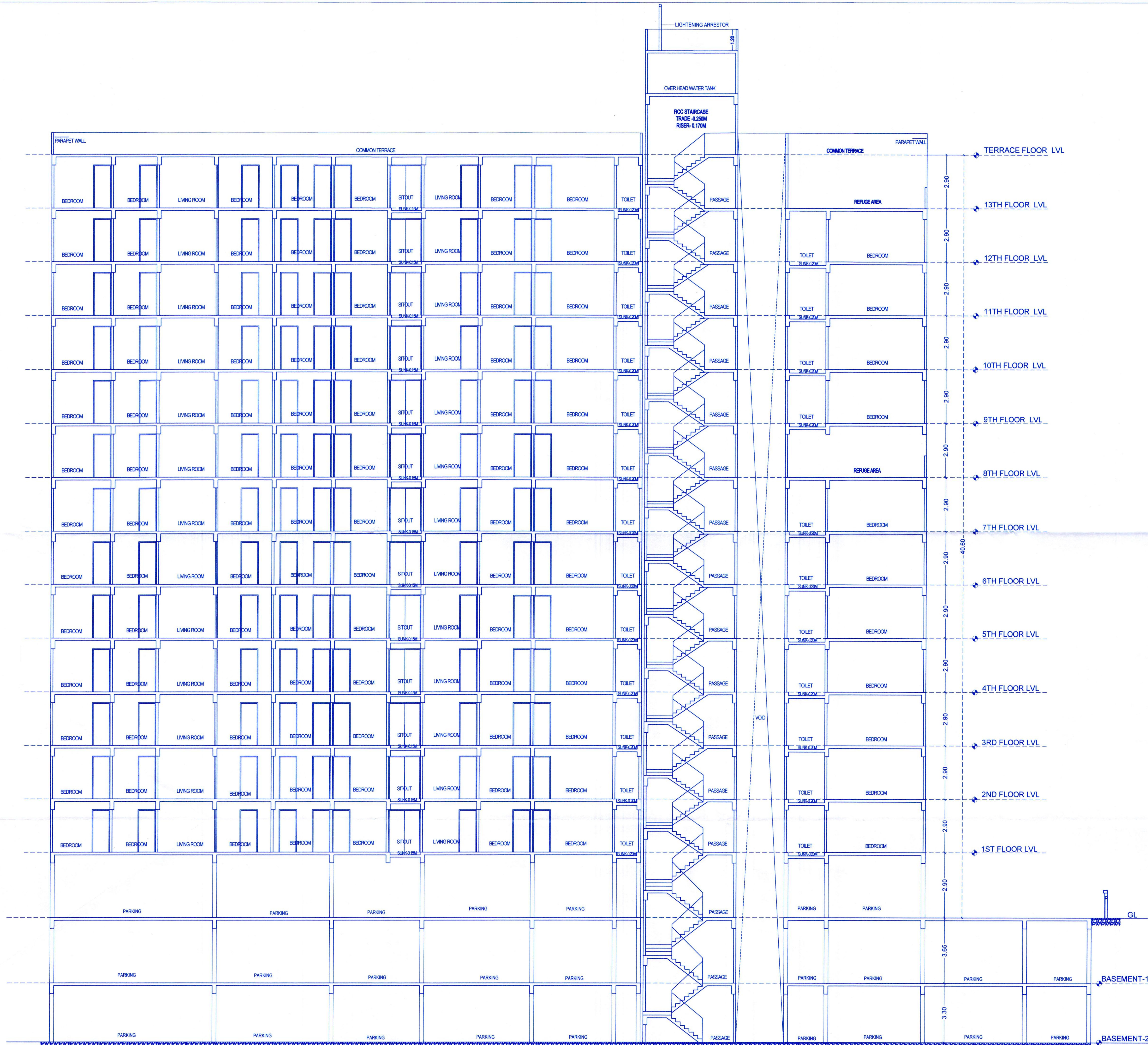
SECTION AT BB' SCALE: 1:100
