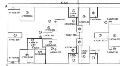
AREA KEY PLAN- EIGHTH FLOOR SCALE 1:100
