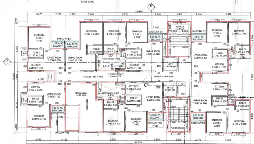
EIGHTH (REFUGE) FLOOR PLAN SCALE 1:100
